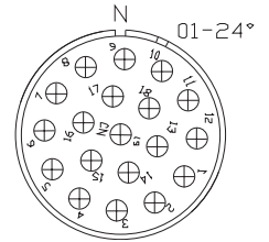
CN-08-377 19 #12 Contacts
