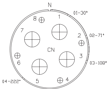
CN-C12-353 4 #12 & 4 #1/0 Contacts
