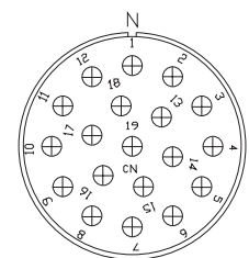
CN-10-376 19 #12 Contacts
