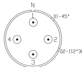
CN-08-328 4 #8 Contacts
