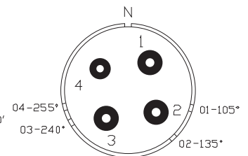
CN-08-22 4 #4 Contacts
