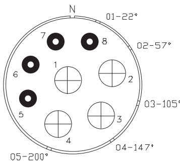
CN-12-355 4 #4 & 4 #1/0 Contacts
