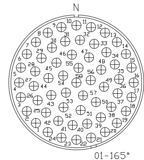
CN-12-384 58 #12 Contacts
