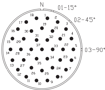
CN-12-371 37 #16 Contacts
