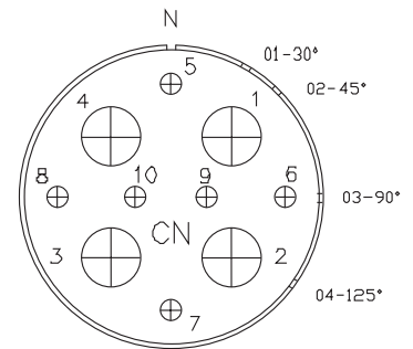
CN-C12-375 6 #12 & 4 #1/0 Contacts
